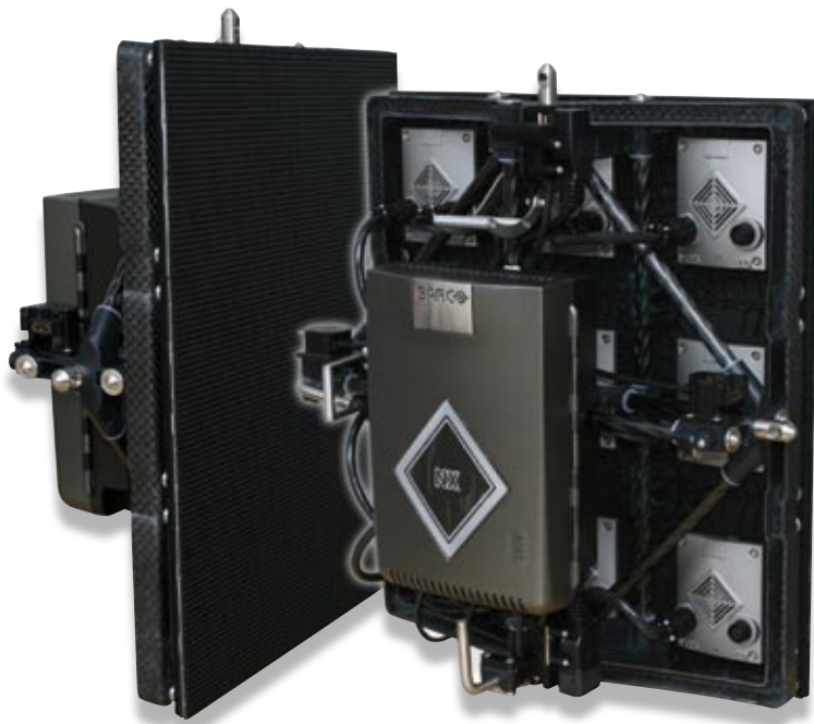
Control unit can be opened while the tile is operational. The same control unit is used on both NX-6 and NX-4.
